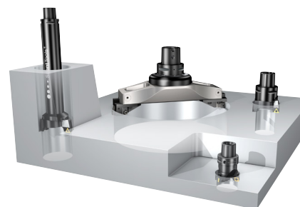
Productive boring
