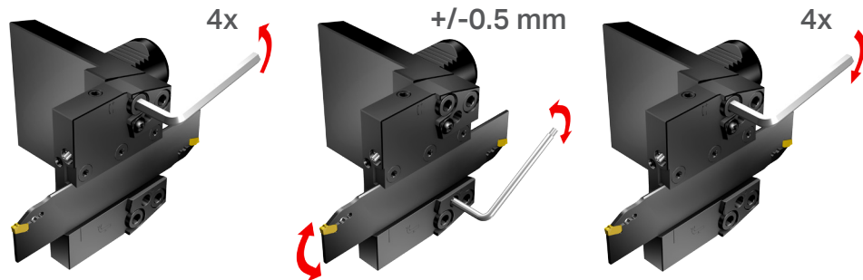
Center height adjustment
