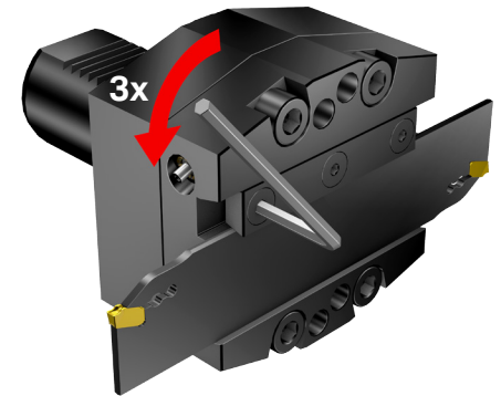
Unclamp the blade
